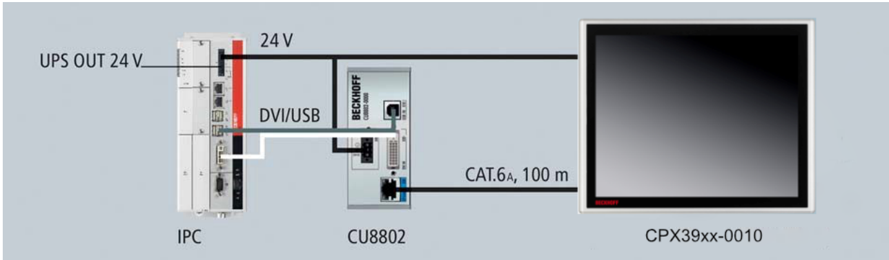
Fig. 4: CP-Link 4-Two cable display link via the CU8802 transmitter box
