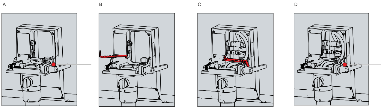
Fig. 29: Cable routing procedure
