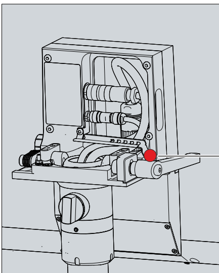
Fig. 35: Releasing the strain relief rail
