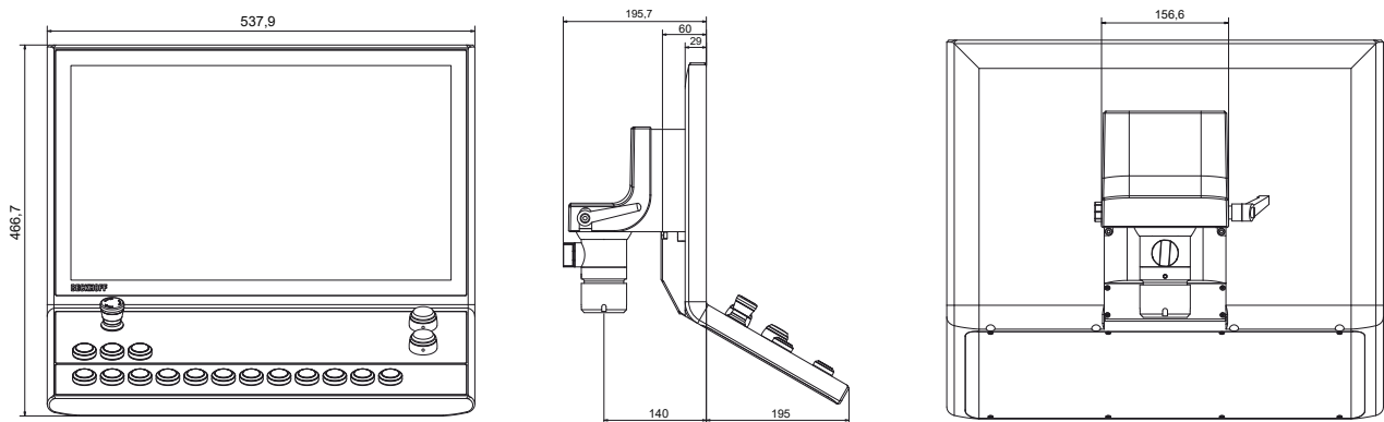
Fig. 24: Dimensions
