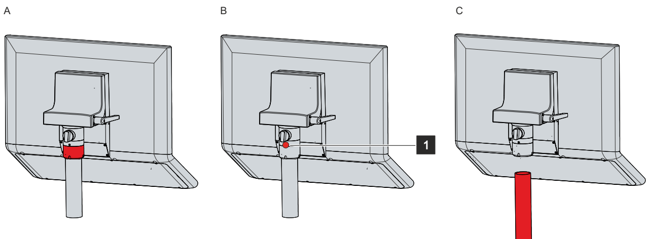
Fig. 36: Disassembly mounting arm tube
