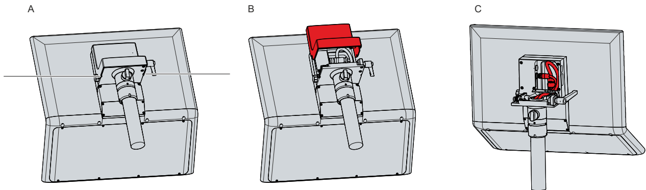
Fig. 11: Access to interfaces
