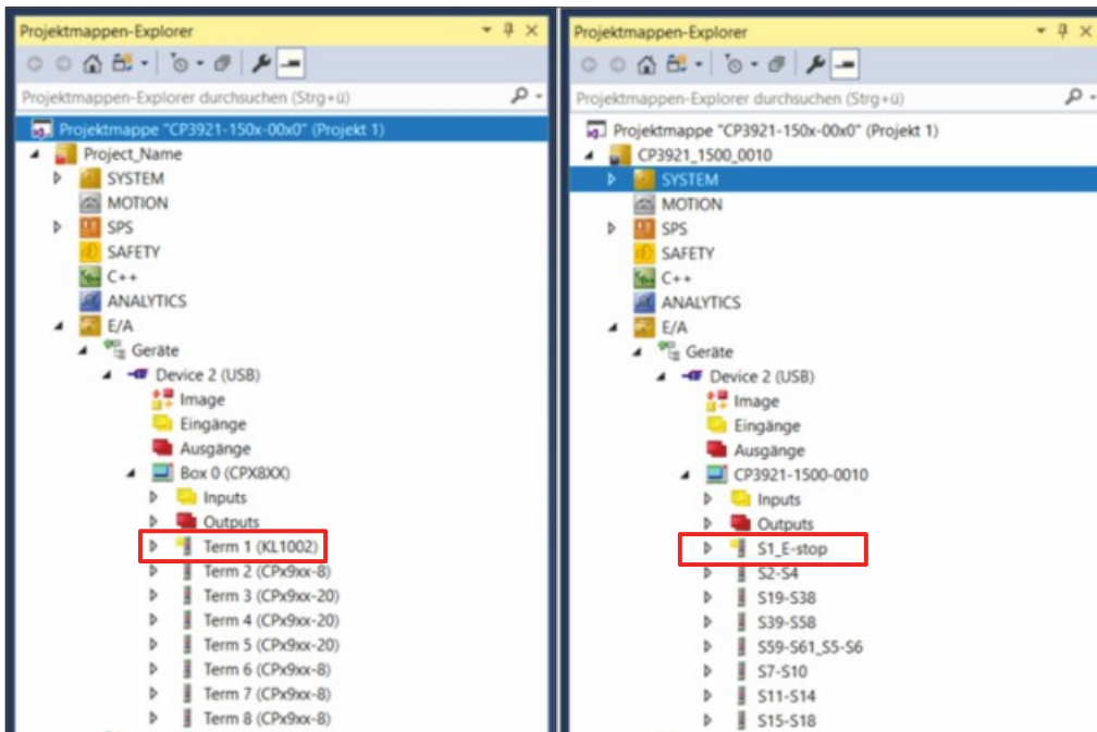
Fig. 34: Rename
