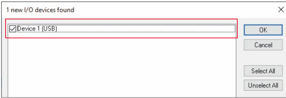
Fig. 32: Select device
