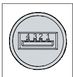
Fig. 10: USB interface pin numbering
