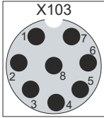
Fig. 8: USB-E input pin numbering
