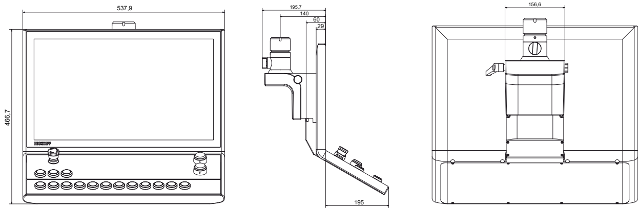
Fig. 25: Dimensions
