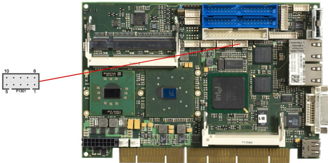
Pinout SMBus/I2C connector:
