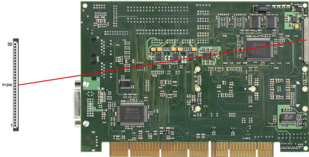
Pinout LVDS connector:
