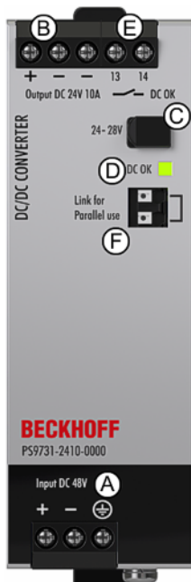
Abb. 13: Front PS9731-2410-0000
