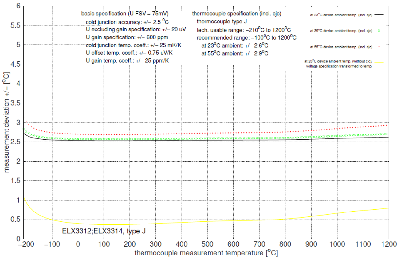
Fig. 35: Measurement uncertainty for type J thermocouple
