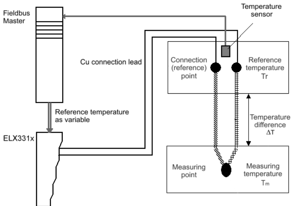
Fig. 45: External cold junction
