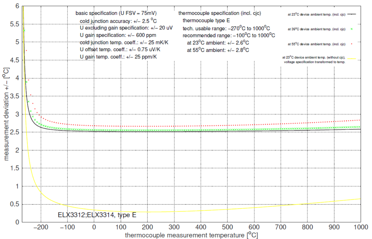
Fig. 34: Measurement uncertainty for type E thermocouple
