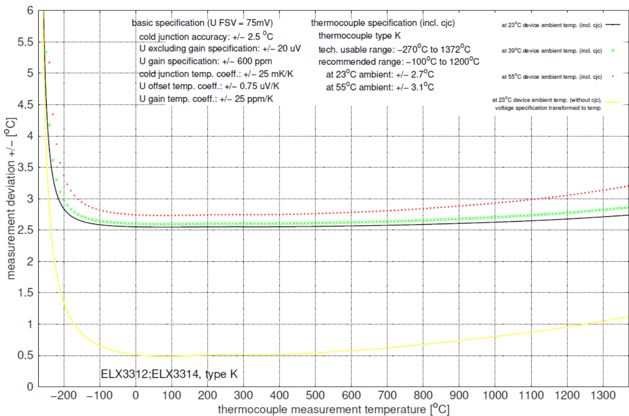
Fig. 36: Measurement uncertainty for type K thermocouple
