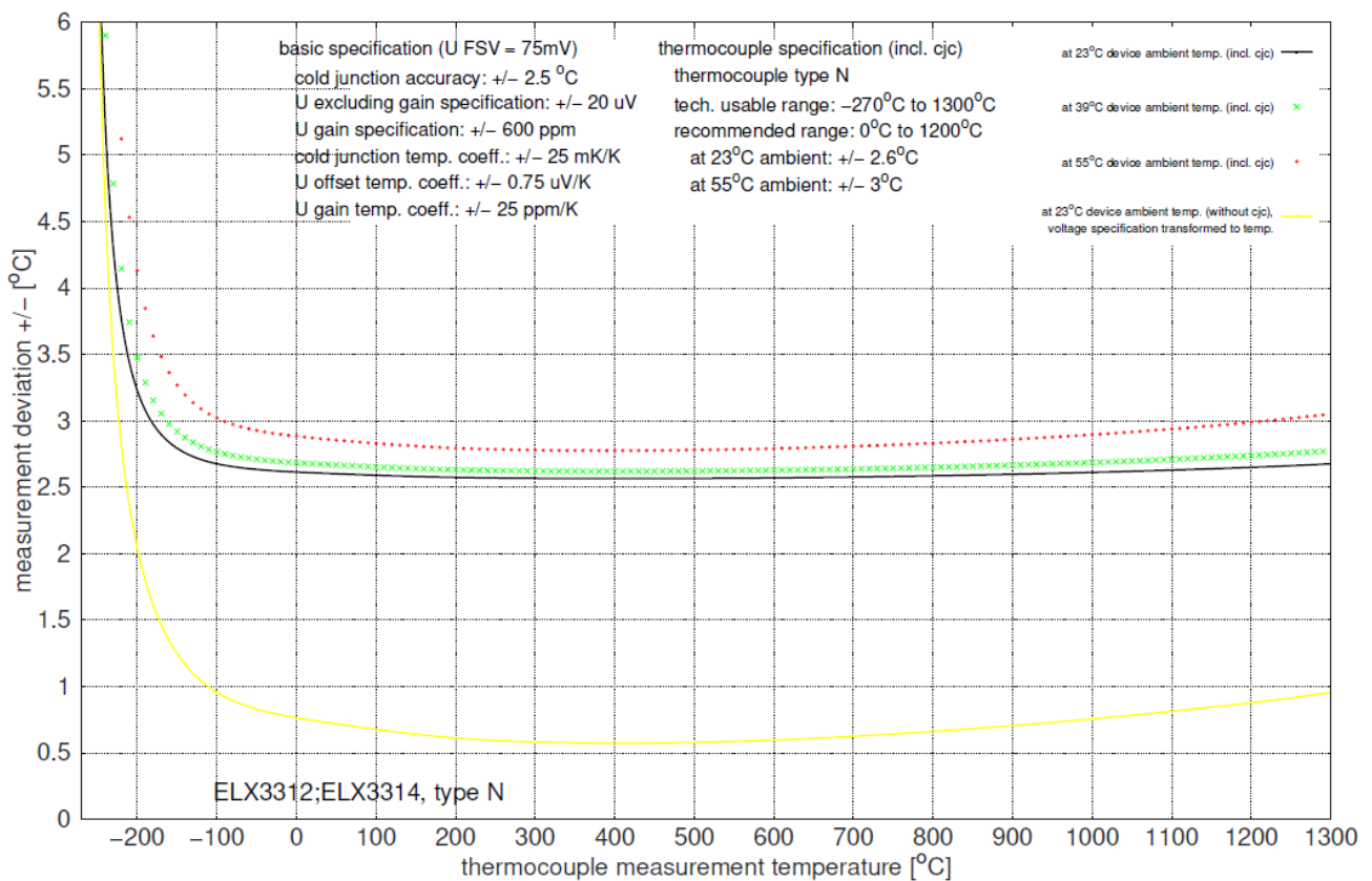
Fig. 38: Measurement uncertainty for type N thermocouple
