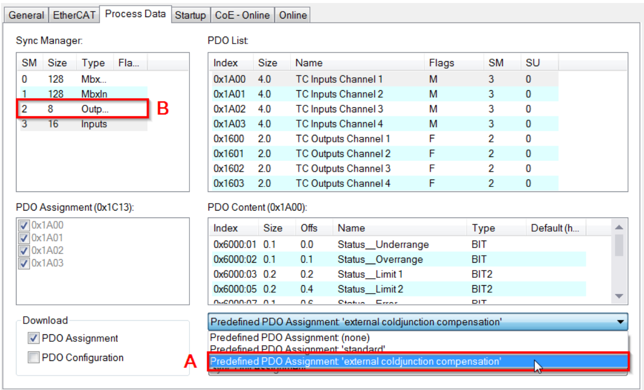
Fig. 51: TwinCAT System Manager with the predefined PDO selection External Compensation
