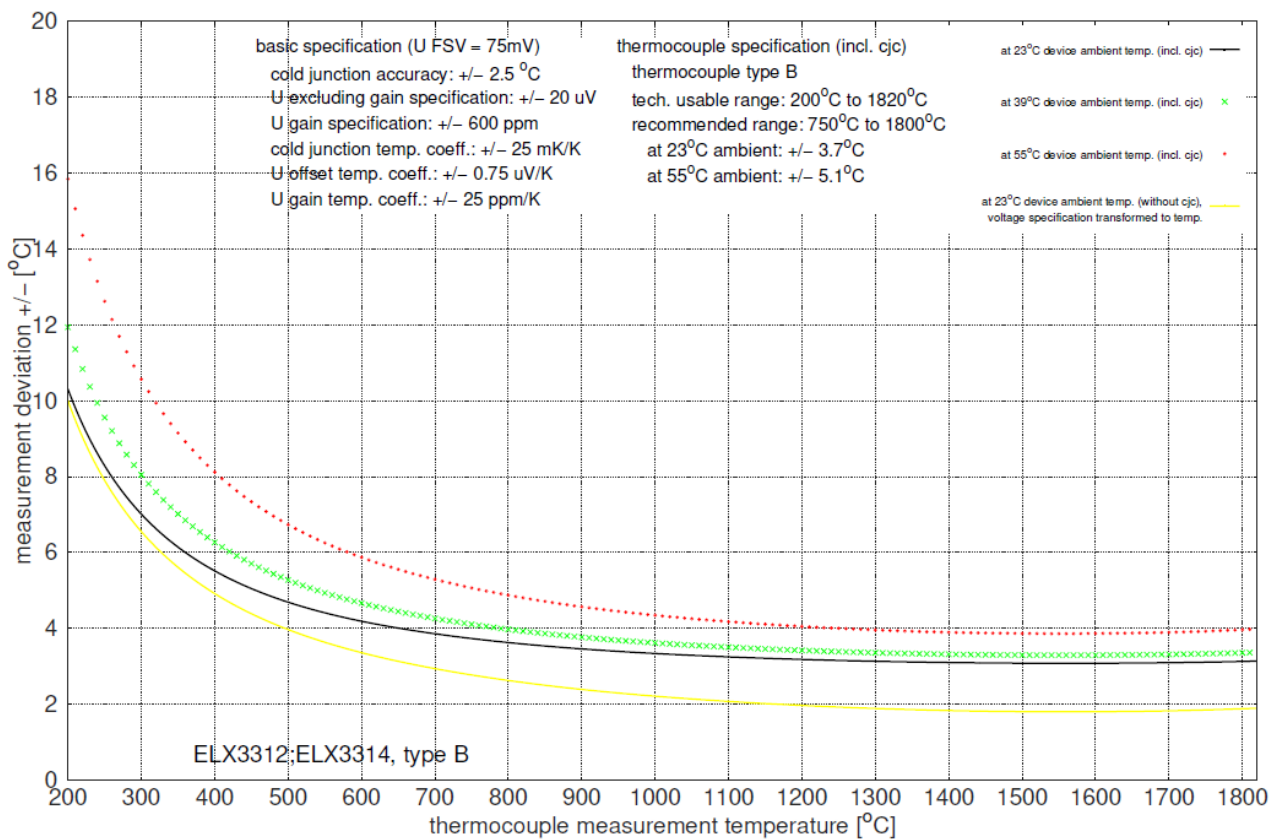
Fig. 32: Measurement uncertainty for thermocouple type B
