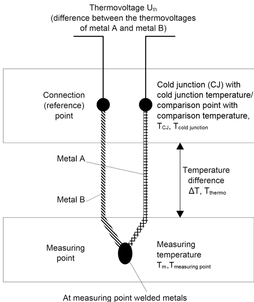
Fig. 31: Principle of the thermocouple
