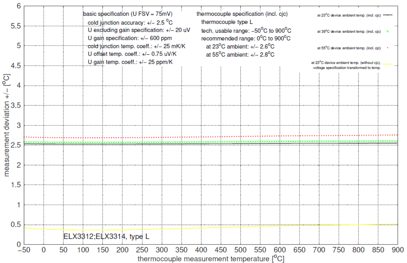
Fig. 37: Measurement uncertainty for type L thermocouple
