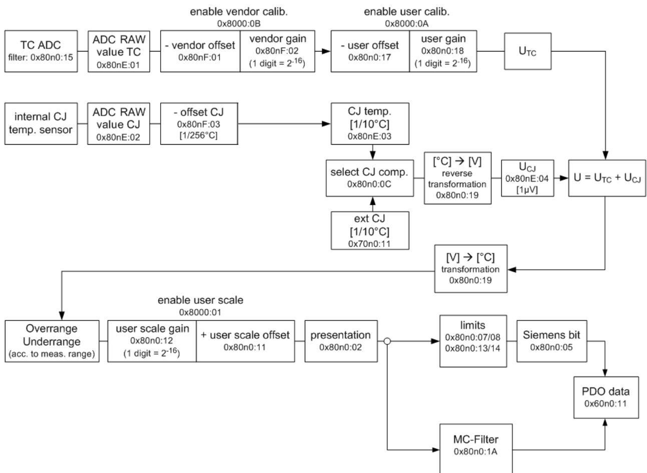
Fig. 43: ELX331x - Data flow
