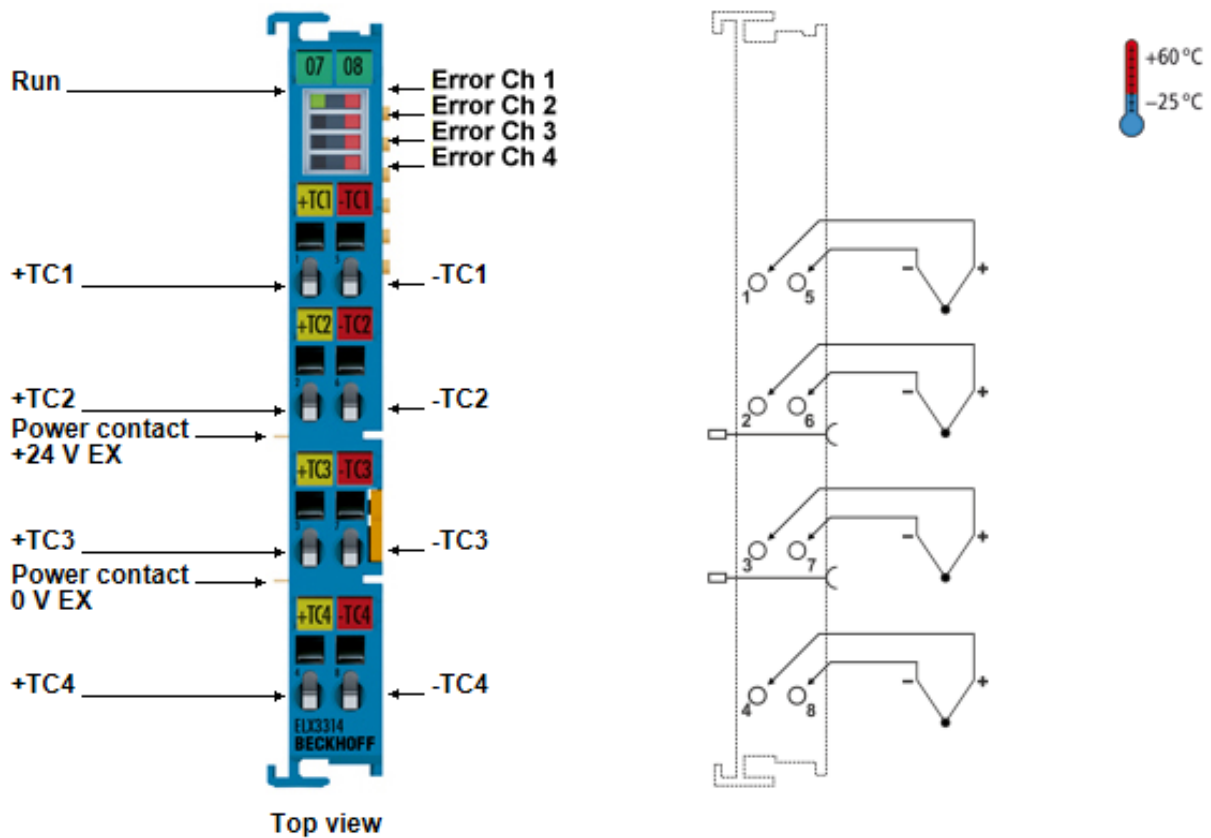
Fig. 22: ELX3314 - Contact assignment
