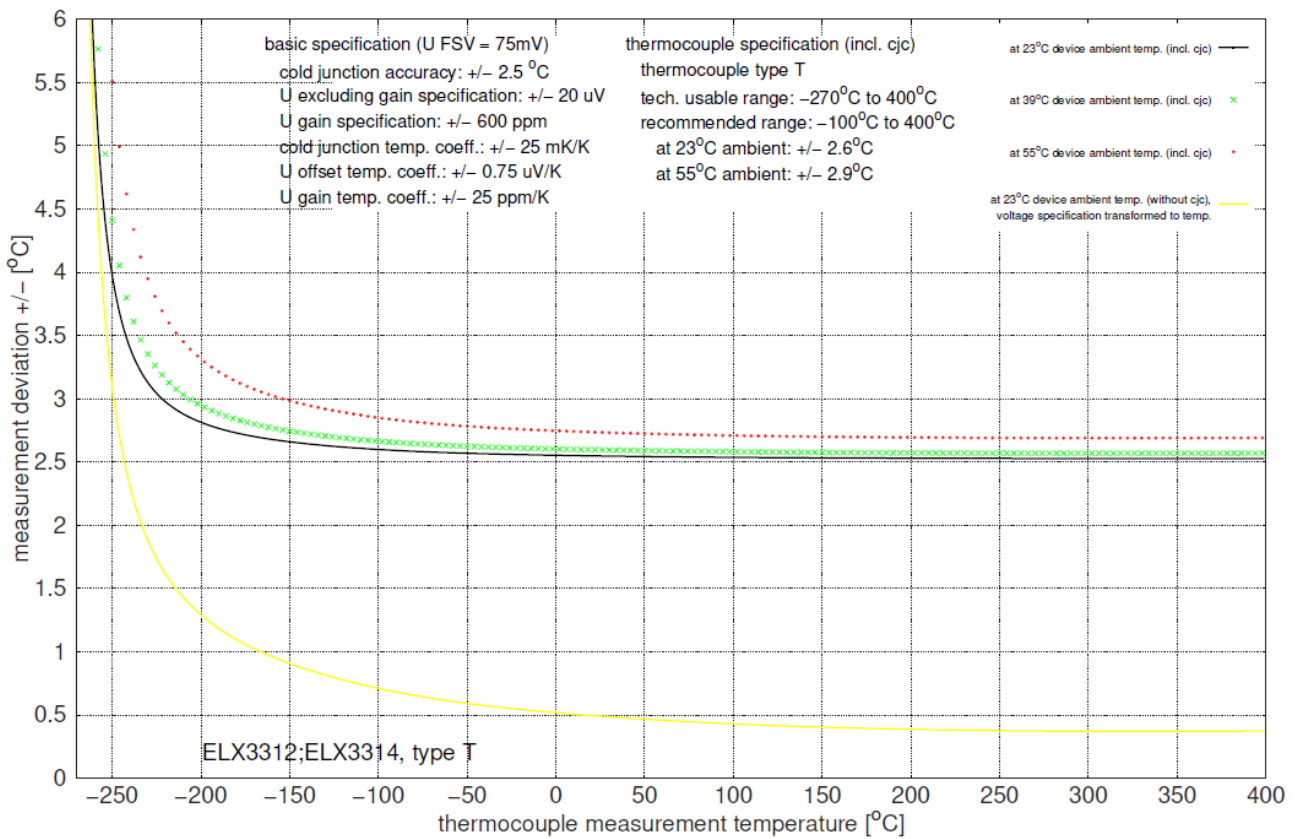
Fig. 41: Measuring uncertainty for type T thermocouple
