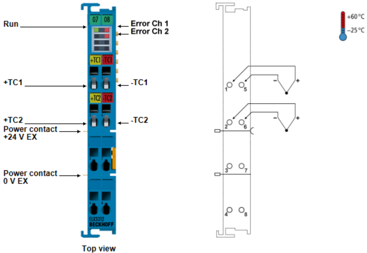
Fig. 21: ELX3312 - Contact assignment
