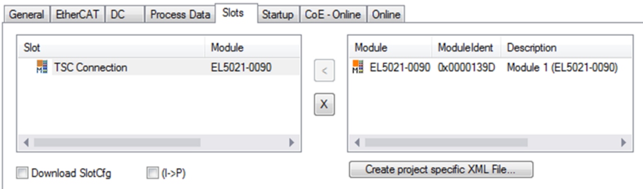
Fig. 52: Adding the TwinSAFE SC process data under the component, e.g. EL5021-0090
