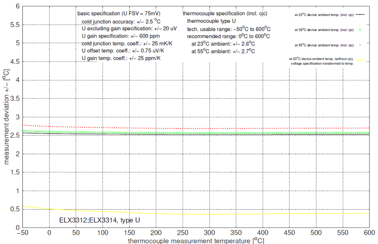
Fig. 42: Measuring uncertainty for type U thermocouple
