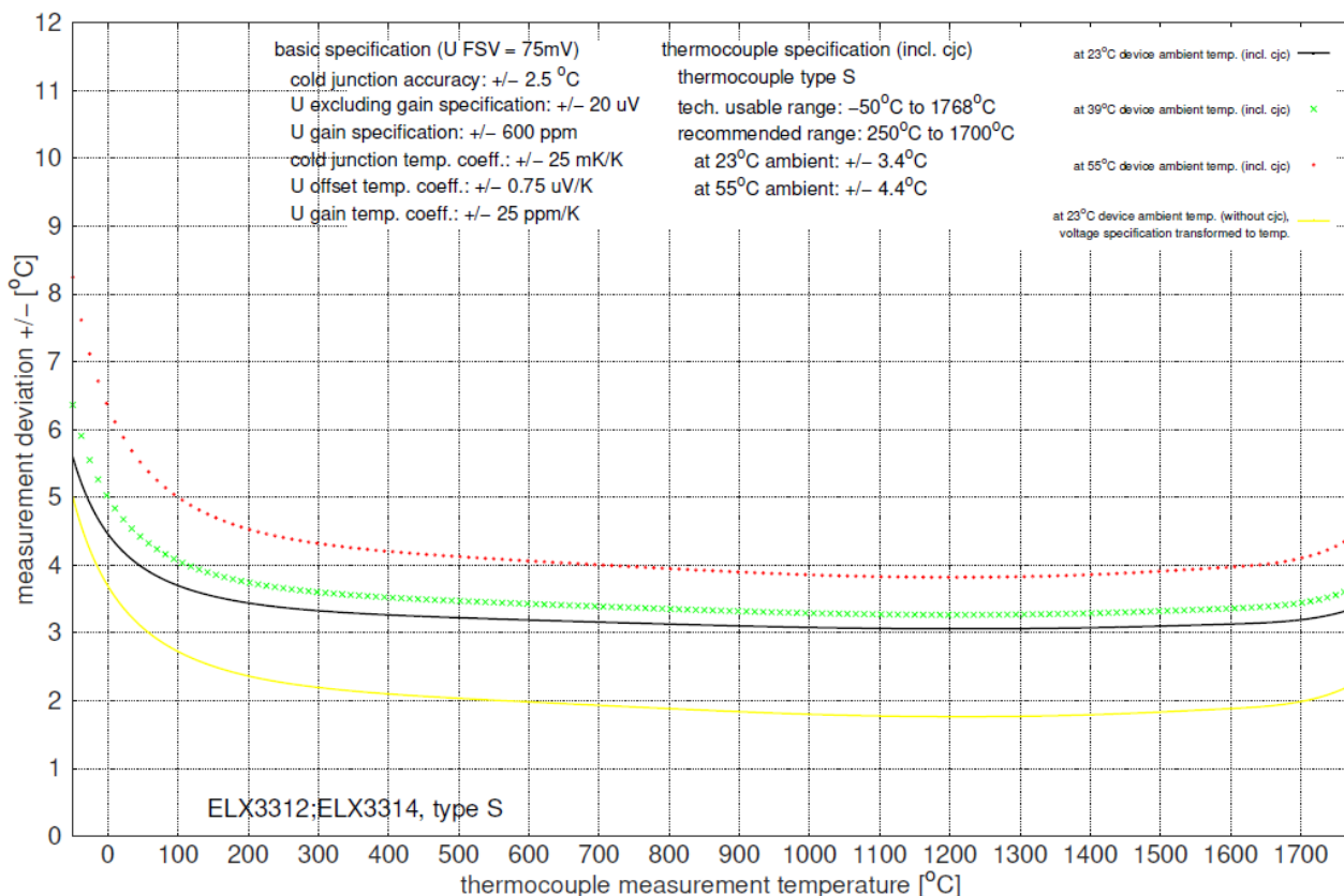
Fig. 40: Measurement uncertainty for type S thermocouple
