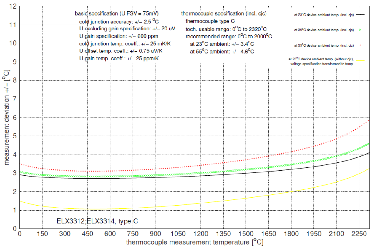
Fig. 33: Measurement uncertainty for thermocouple type C
