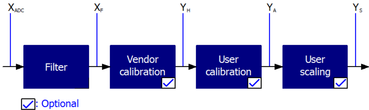
Fig. 44: Calculation of process data
