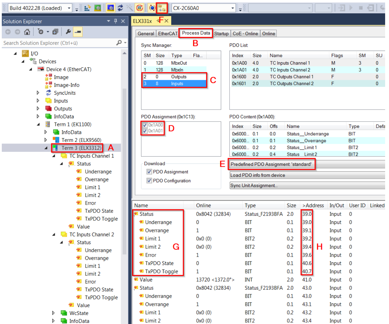
Fig. 47: ELX3312 – Process data selection in TwinCAT
