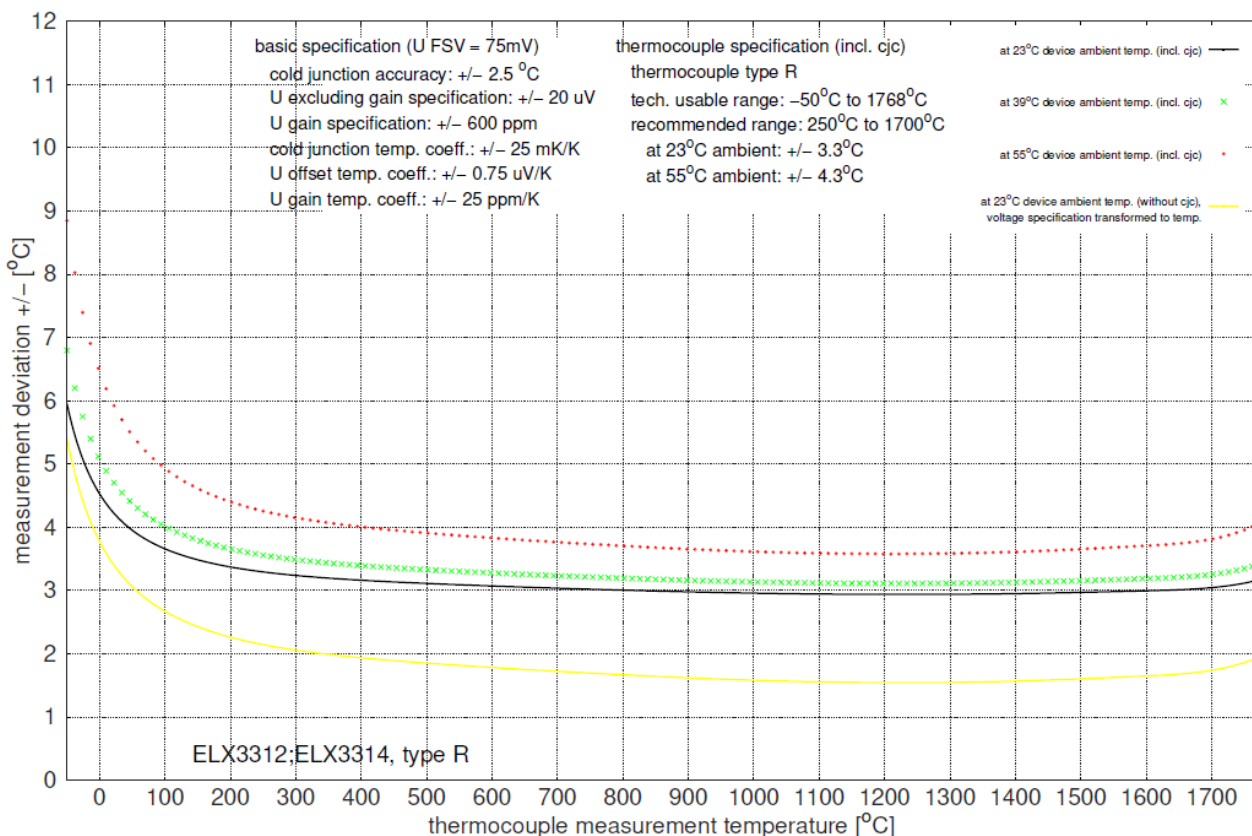
Fig. 39: Measurement uncertainty for type R thermocouple
