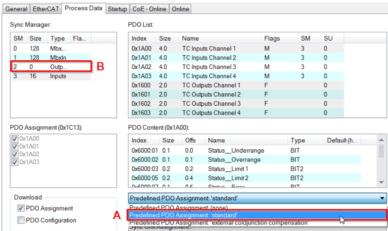
Fig. 50: TwinCAT System Manager with predefined PDO option Standard
