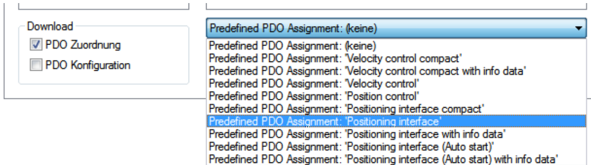
Abb. 178: Predefined PDO Assignment
