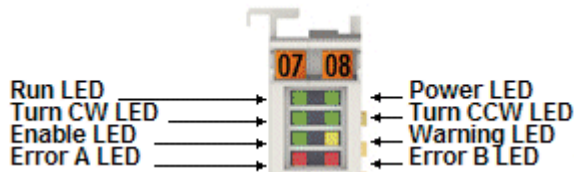
Abb. 30: LEDs EL7031
