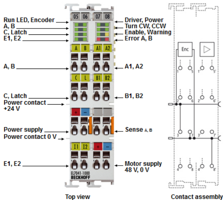
Abb. 7: EL7041-1000
