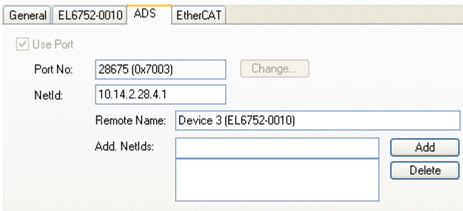
Fig. 34: “ADS” tab
