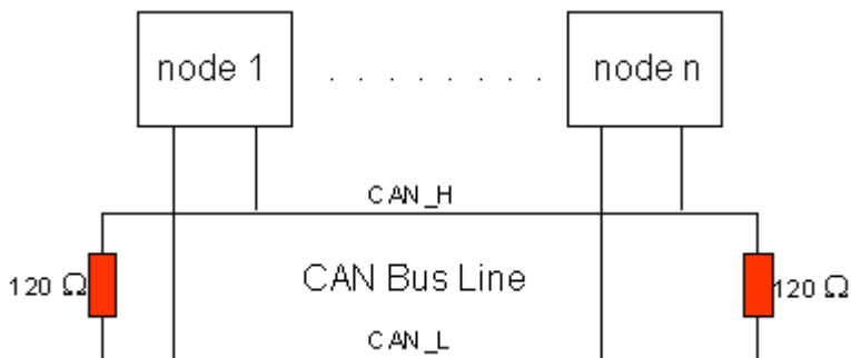
Fig. 8: DeviceNet topology
