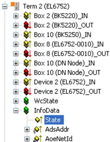
Fig. 67: State diagnostic variable in the TwinCAT tree
