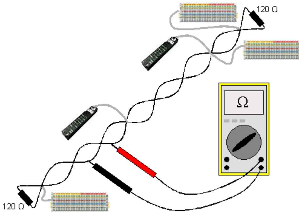
Fig. 143: Wiring diagram for test setup
