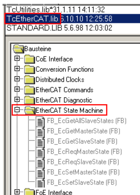
Fig. 81: PLC function blocks
