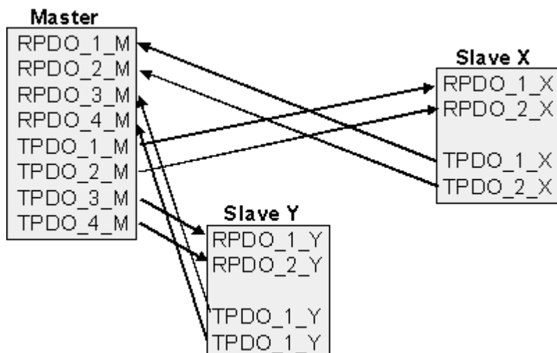
Fig. 109: Default identifier allocation: Master/Slave
