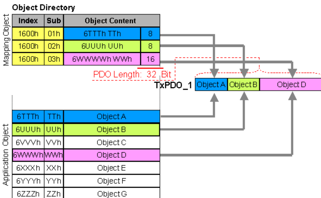
Fig. 115: Mapping representation
