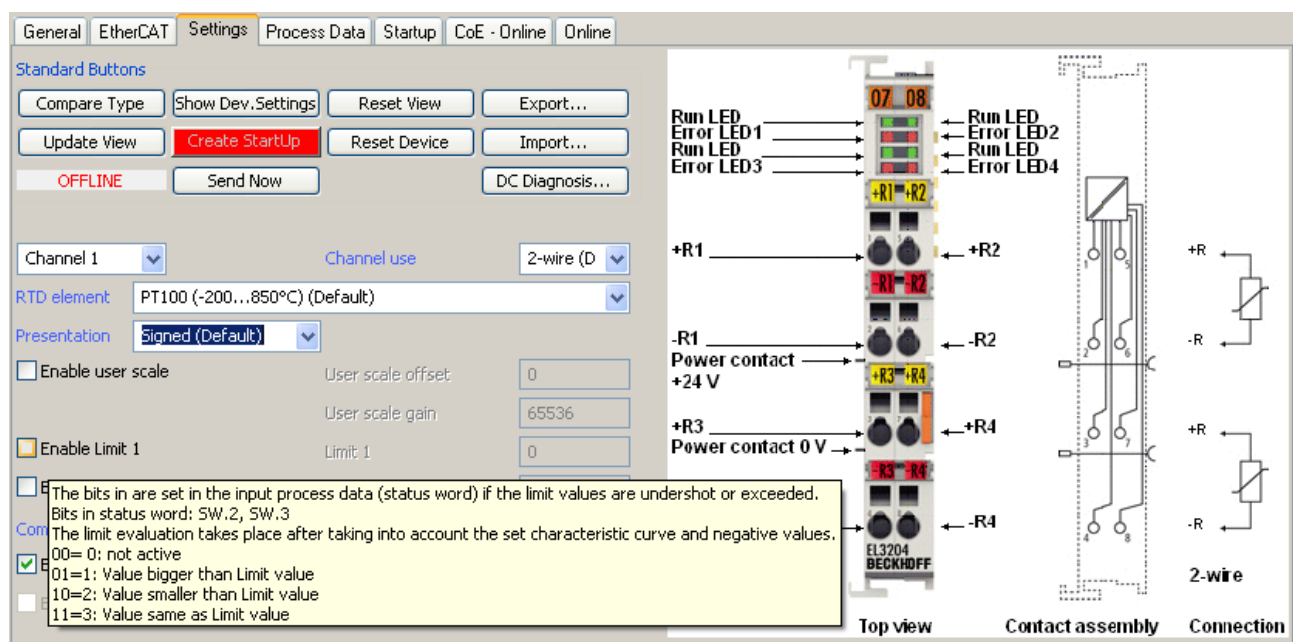
Fig. 78: Example of commissioning aid for a EL3204
