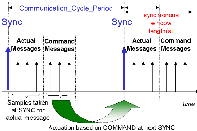
Fig. 112: Diagram: CAN "SYNC" telegram
