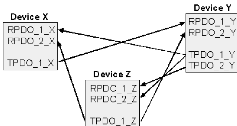
Fig. 110: PDO linking: Peer to Peer
