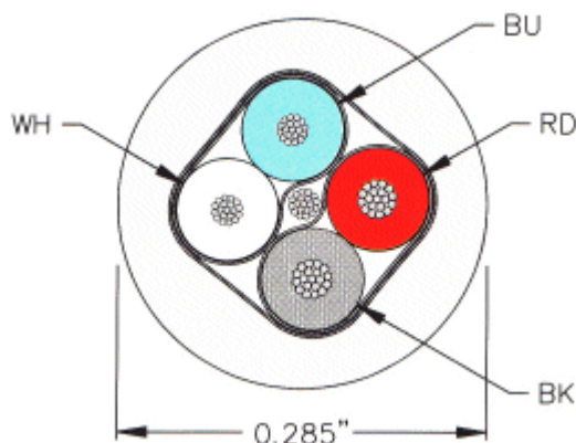
Fig. 16: Structure of CAN/DeviceNet cable ZB5200
