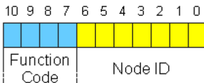
Fig. 119: Schematic: CANopen default identifier
