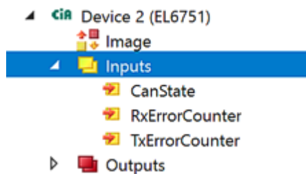
Fig. 128: Minimum diagnosis
