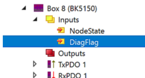
Fig. 123: Variable DiagFlag
