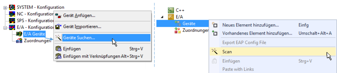
Abb. 112: Scan Devices (links: TwinCAT 2; rechts: TwinCAT 3)
