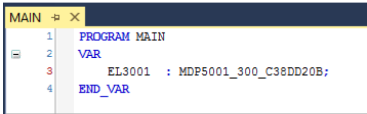
Abb. 80: Instance_of_struct
