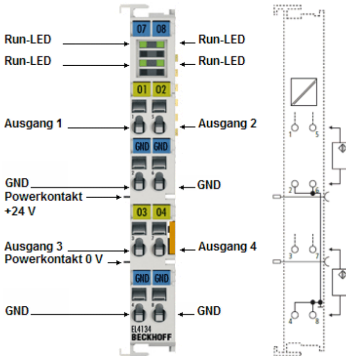
Abb. 18: EL4134-00xx
