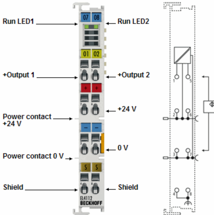
Abb. 8: EL4112-00xx
