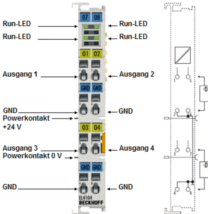
Abb. 6: EL4104
