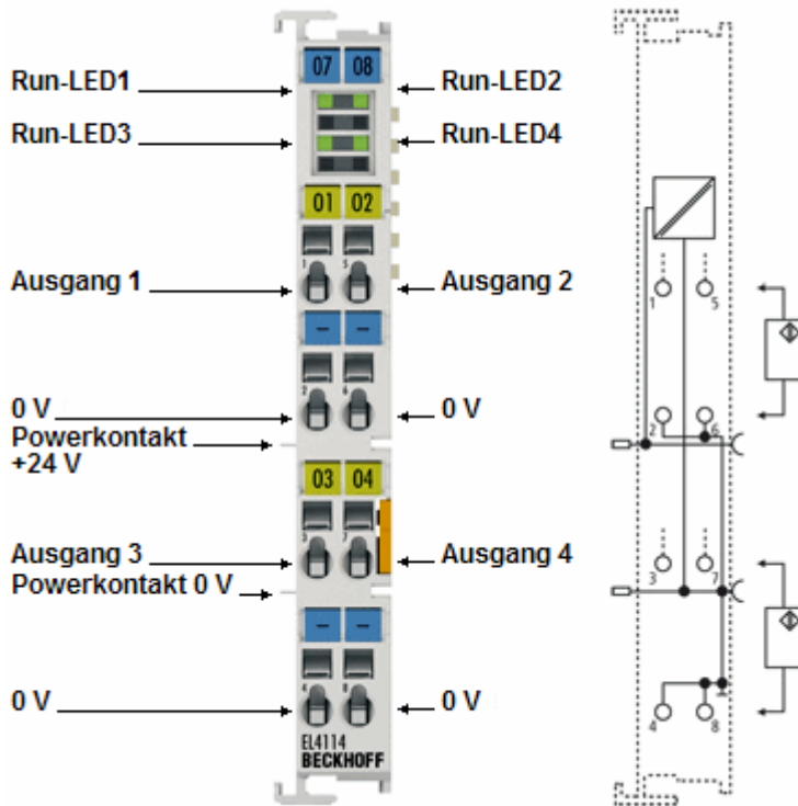
Abb. 10: EL4114-xxxx
