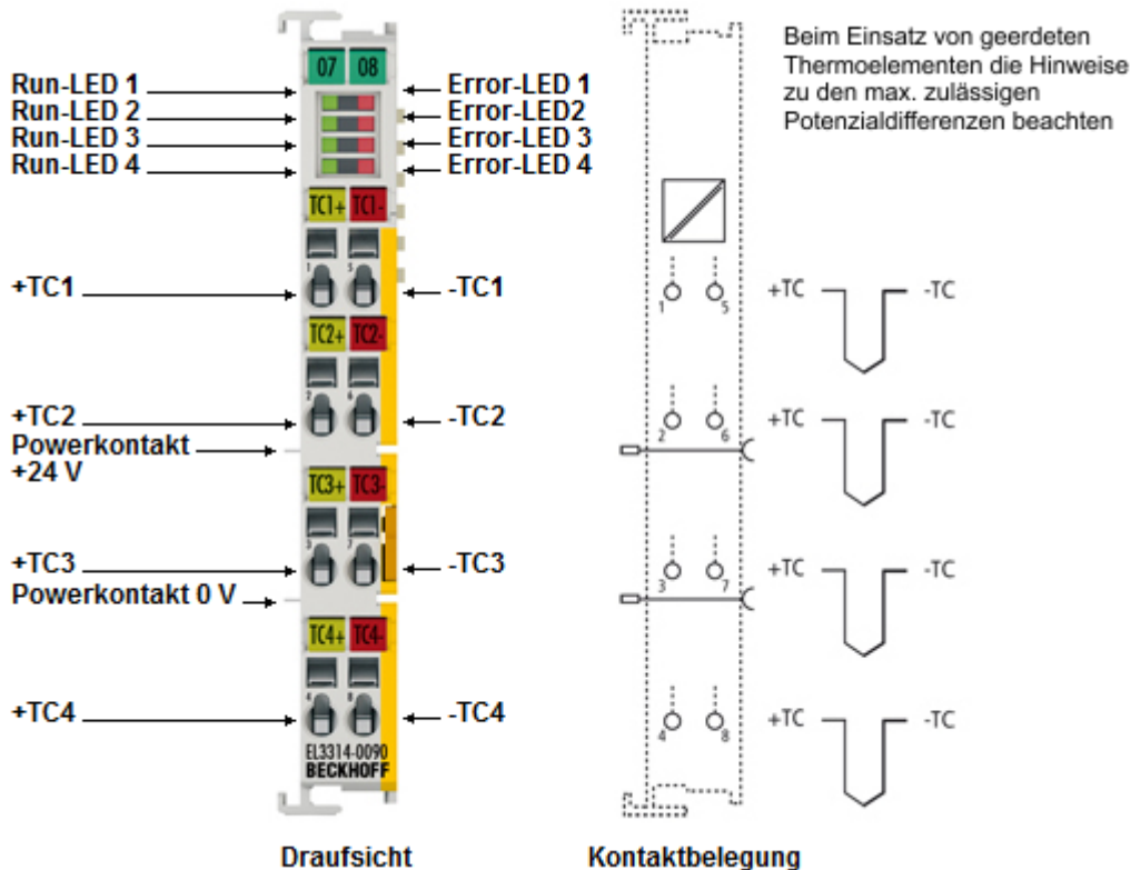
Abb. 62: EL3314-0090
