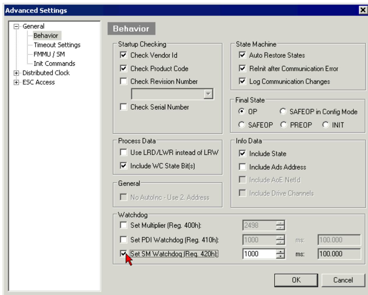
附图 62: EtherCAT 选项卡 -> Advanced Settings -> Behavior-> Watchdog
