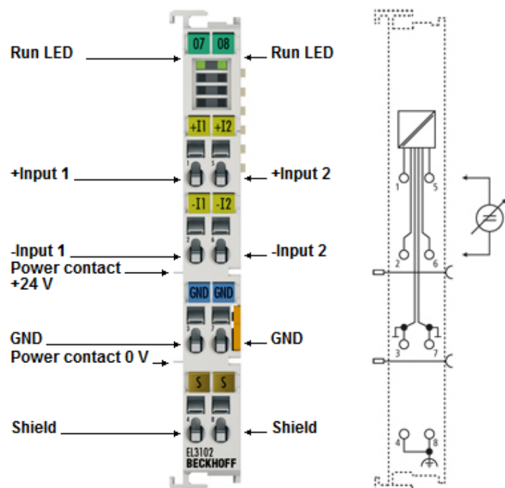
附图 6: EL3102
