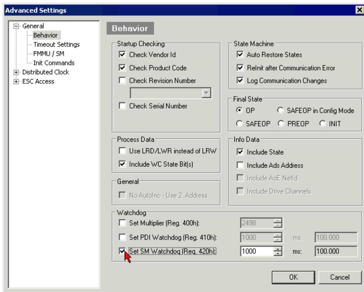
附图 14: EtherCAT 选项卡 -> Advanced Settings -> Behavior-> Watchdog
