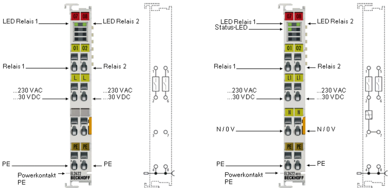
Abb. 10: EL2622, EL2622-0010
