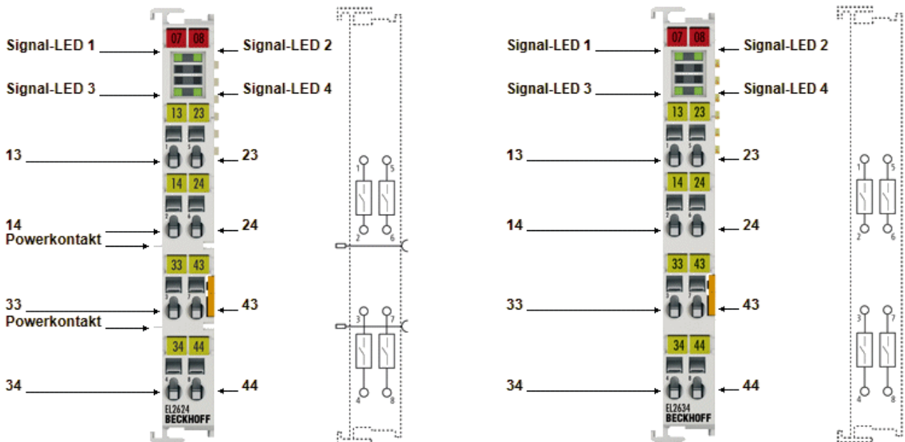
Abb. 11: EL2624, EL2634
