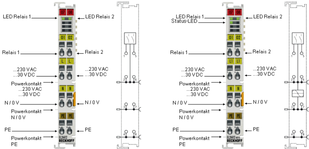
Abb. 4: EL2602, EL2602-0010
