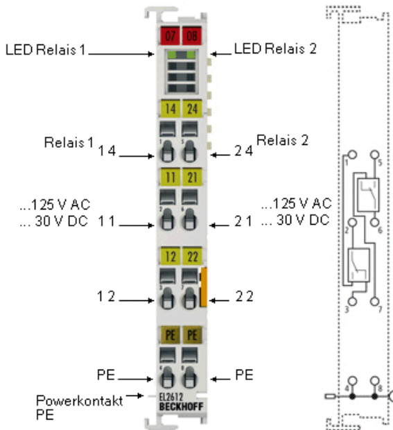
Abb. 7: EL2612
