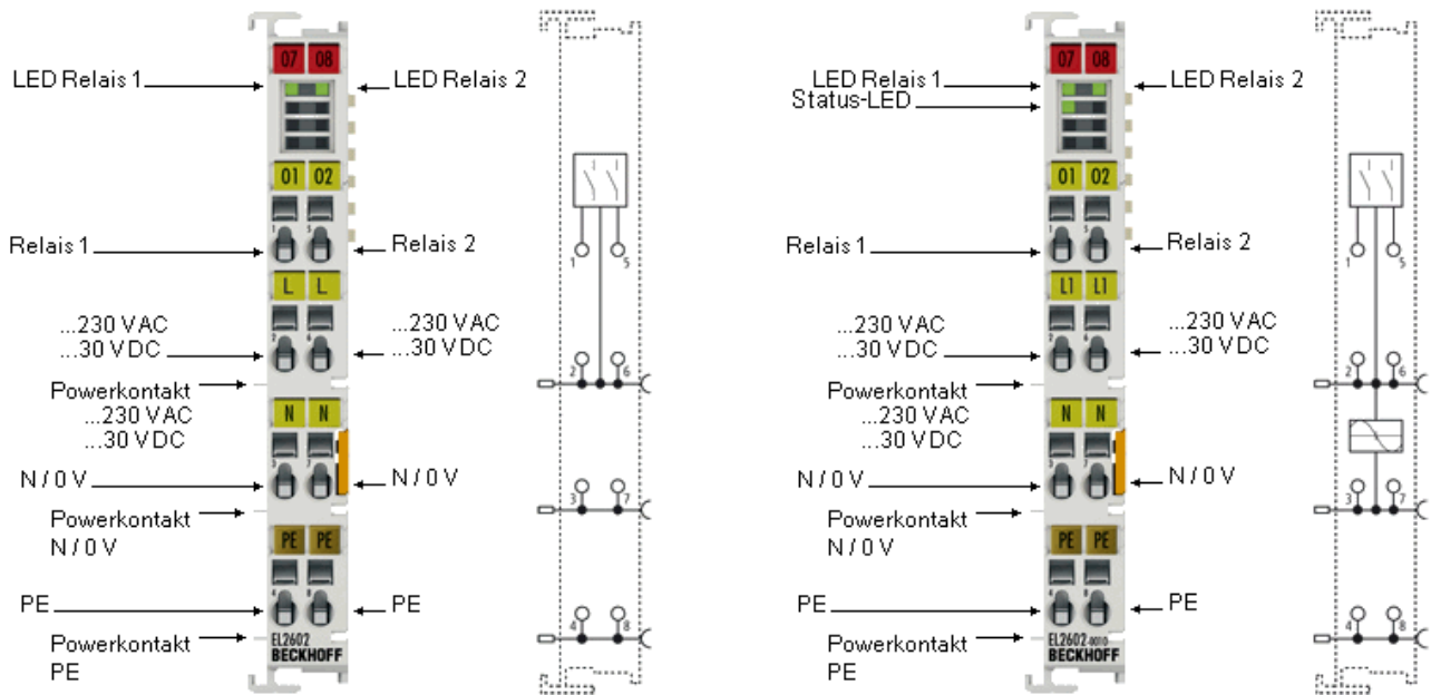
Abb. 5: EL2602, EL2602-0010
