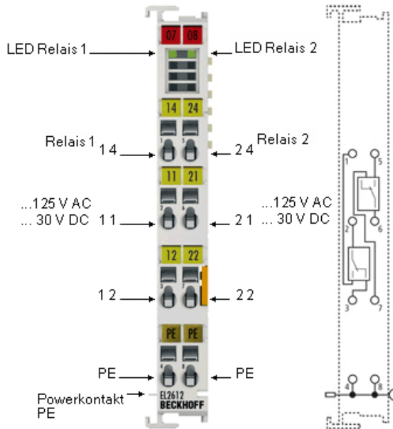
Abb. 6: EL2612
