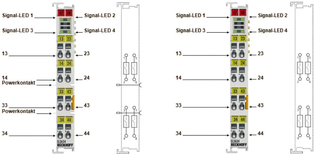
Abb. 9: EL2624, EL2634
