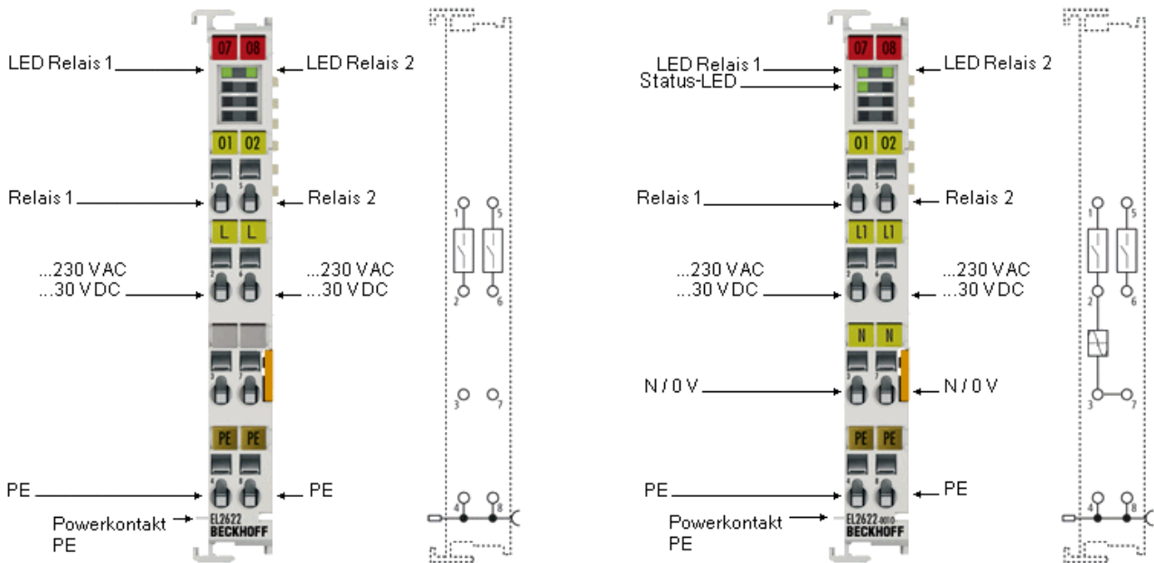
Abb. 8: EL2622, EL2622-0010
