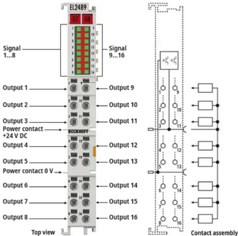
Abb. 7: EL2489
