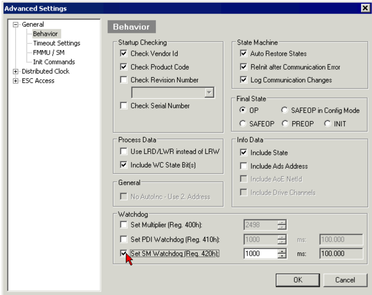
附图 8: EtherCAT 选项卡 -> Advanced Settings -> Behavior-> Watchdog
