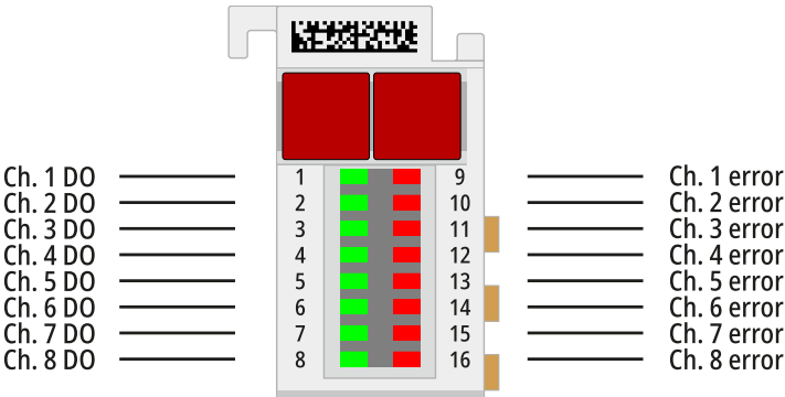
Abb. 7: ED2838 - LEDs
