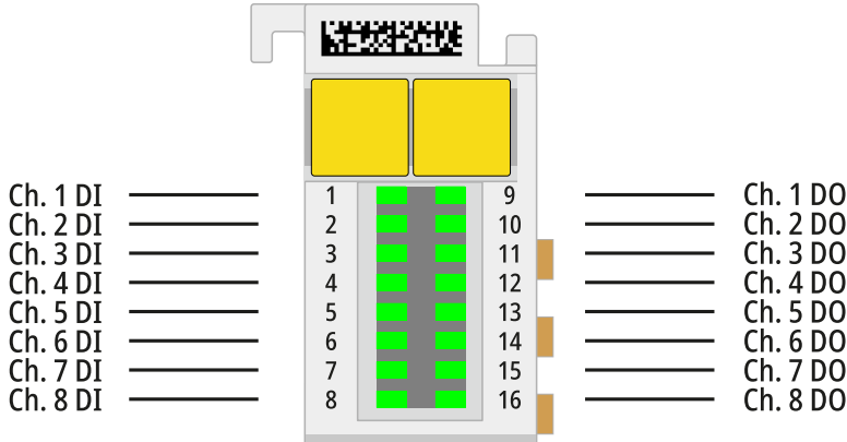
Abb. 5: ED1859 - LEDs
