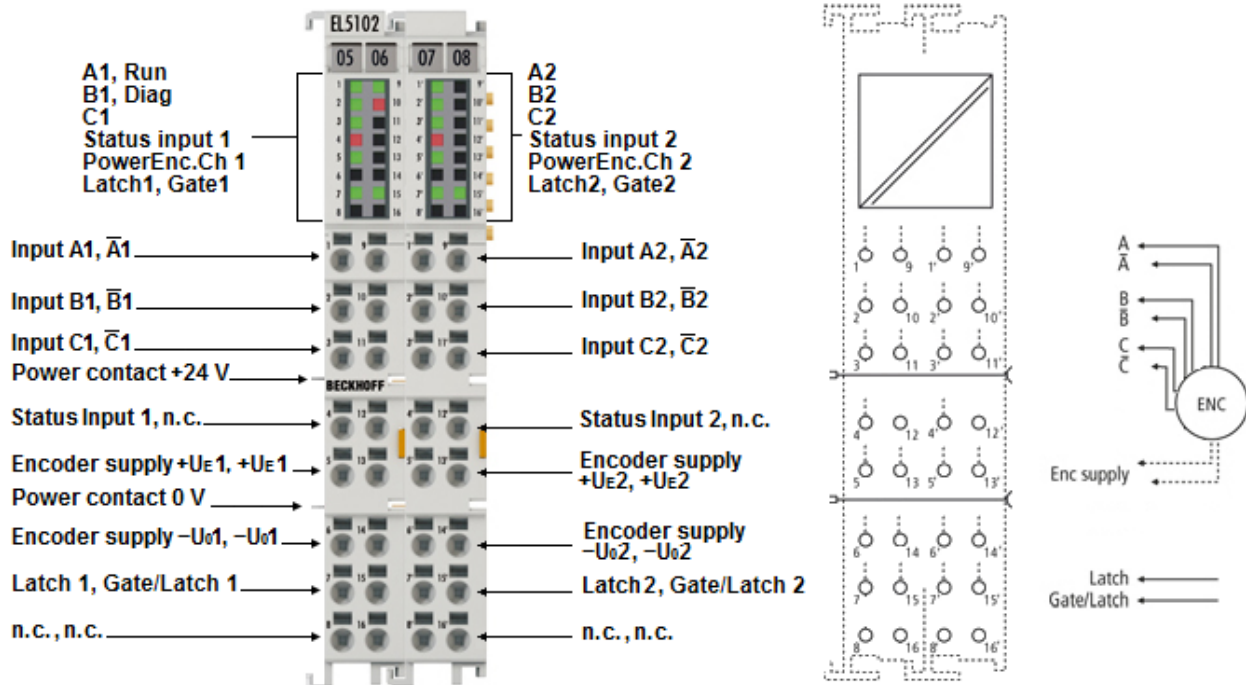
Abb. 4: EL5102
