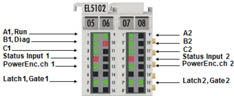
Abb. 34: EL5102 - LEDs
