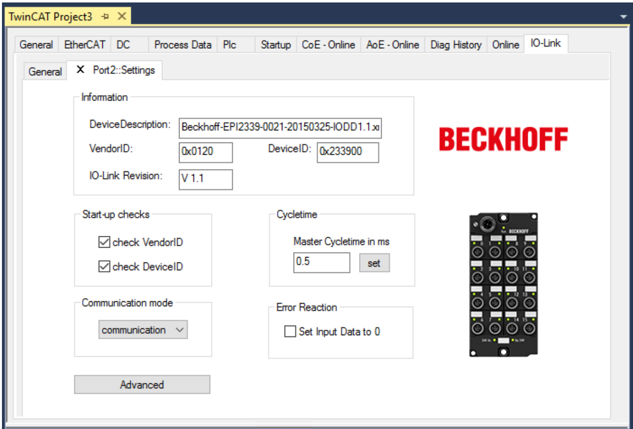
Fig. 17: Settings of the device assigned to port2
