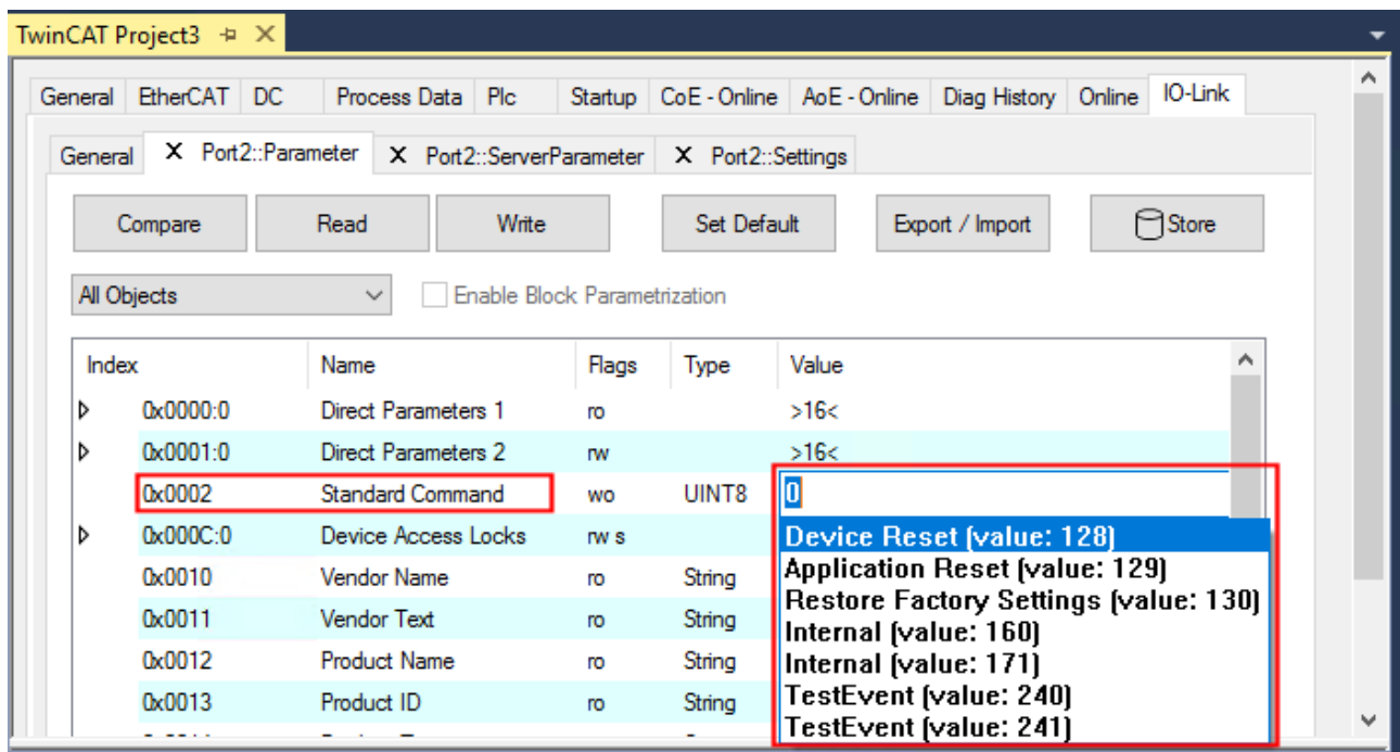
Fig. 34: Parameters IO-Link device “Standard Command”
