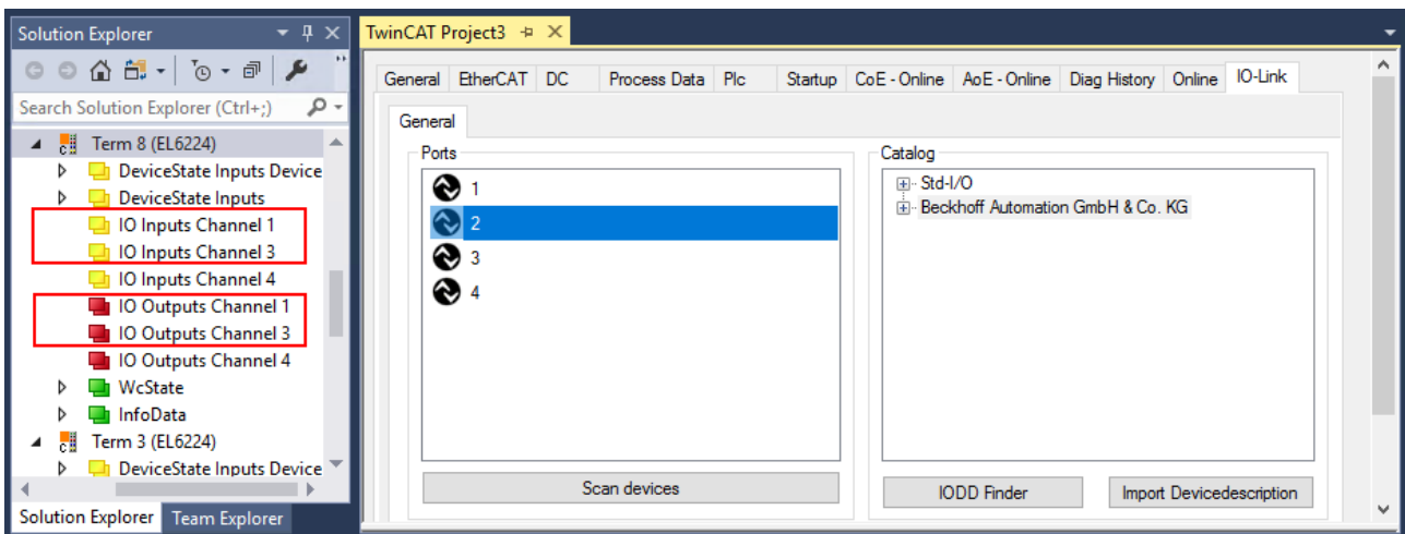
Fig. 21: The device was removed from the port2, the process data no longer displayed in the tree.
