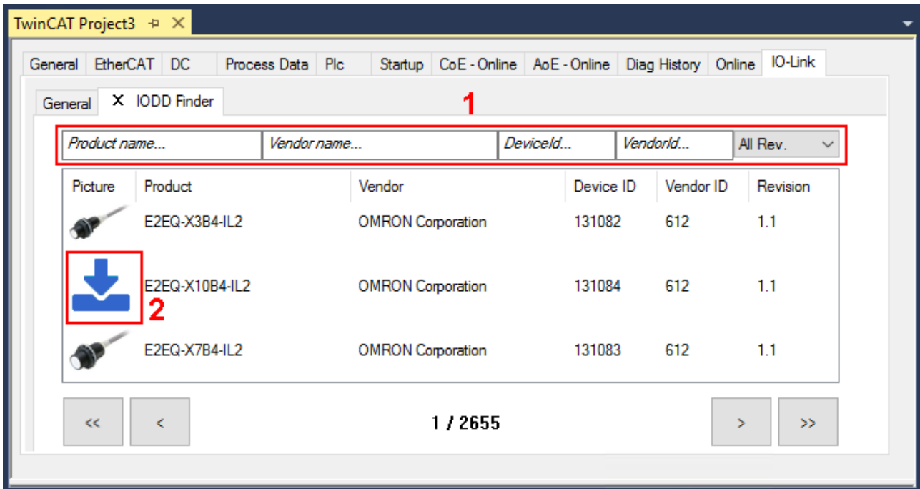
Fig. 12: IODD Finder, selection and import of the .xml-file
