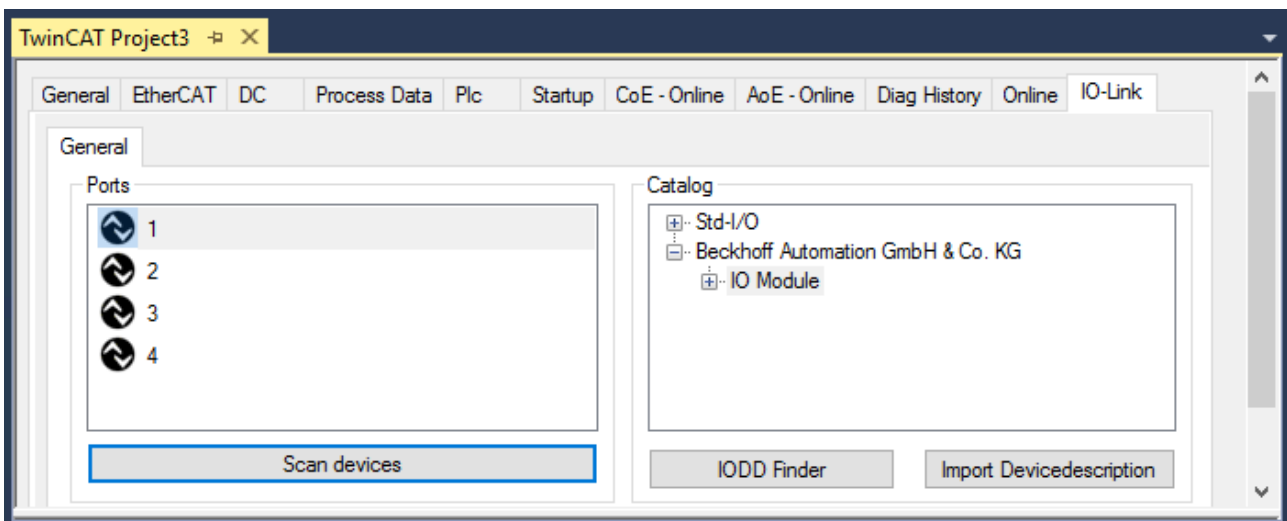
Fig. 14: Scan devices
