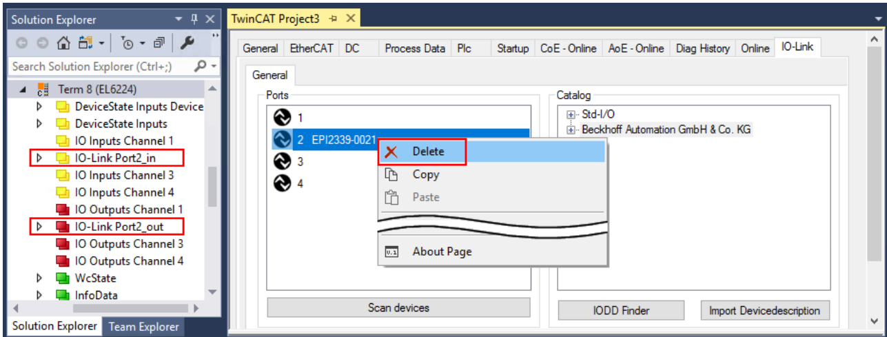
Fig. 20: Remove the device from port2
