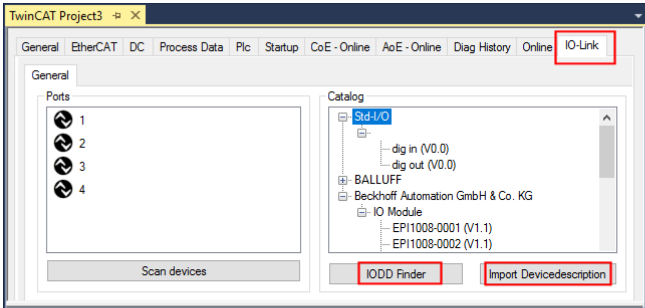
Fig. 11: Import of the IODD device description via “IODD Finder” or “Import Devicedescription”
