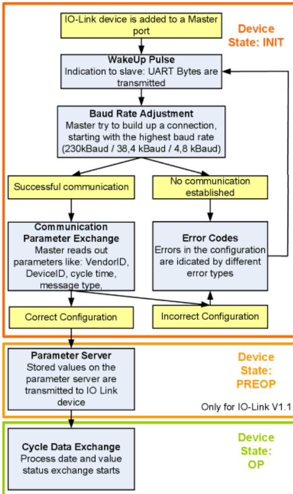
Fig. 1: Establishment of IO Link communication
