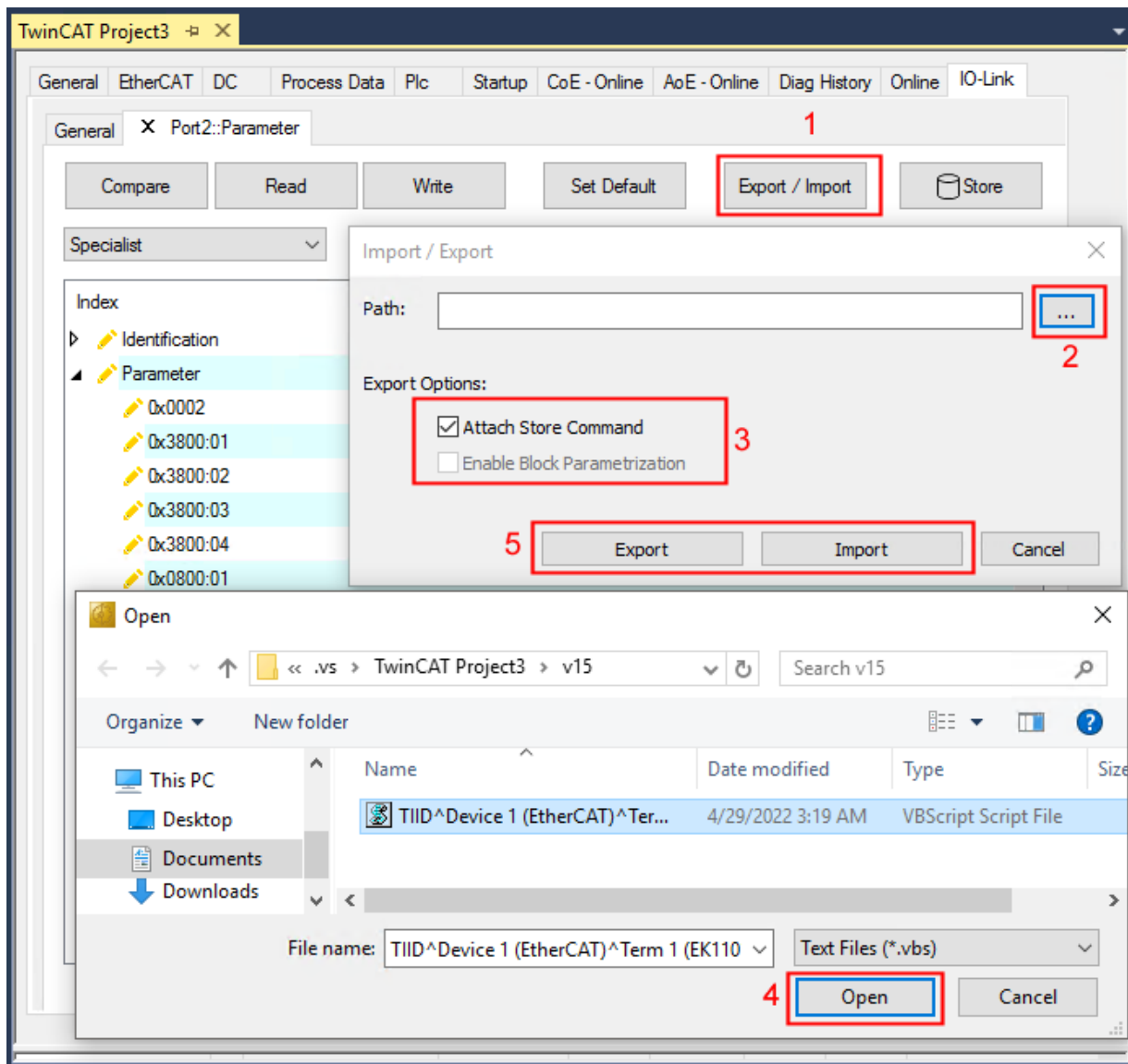
Fig. 29: Parameterization IO-Link device - Export / Import
