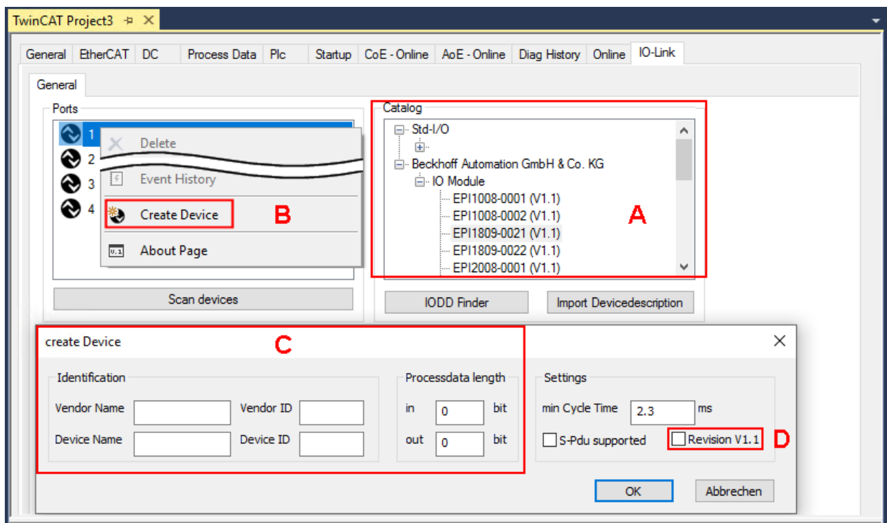
Fig. 19: Manual creation of an IO-Link device via the "Create Device" dialog (C)
