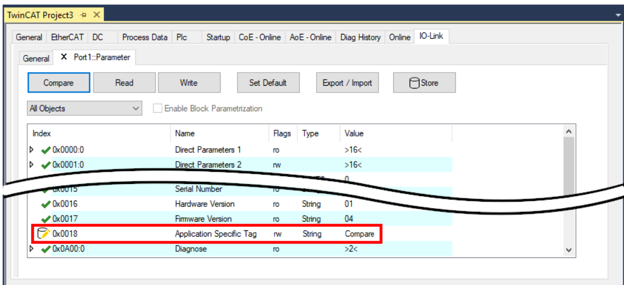
Fig. 25: Display of deviating data in the “Parameter” tab
