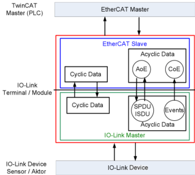
Fig. 36: Illustration of the system communication of an EtherCAT master
