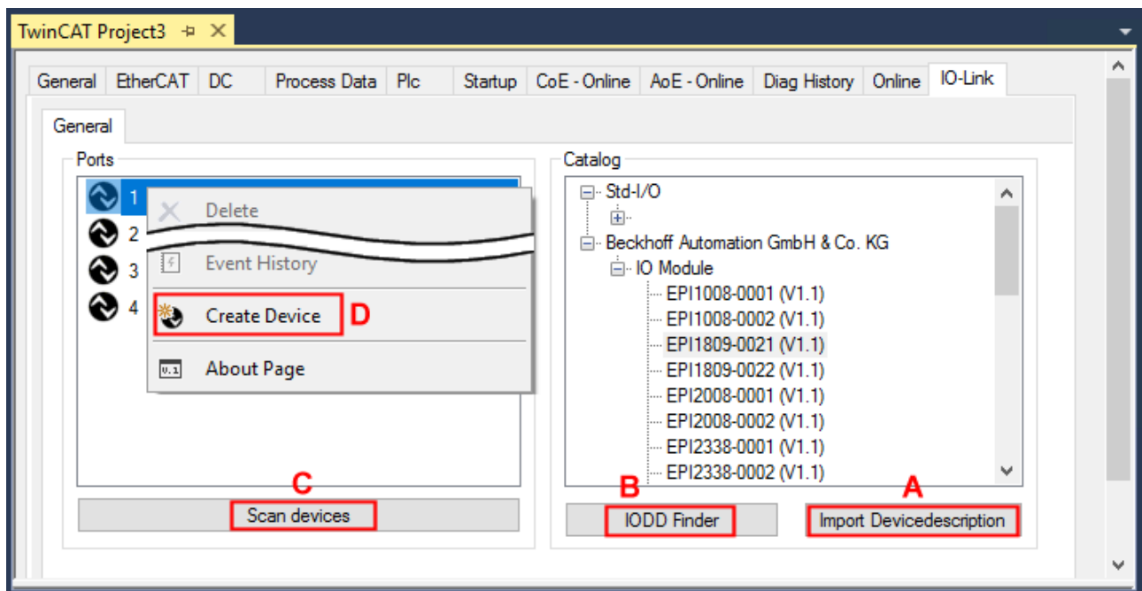
Fig. 10: Creating IO-Link devices
