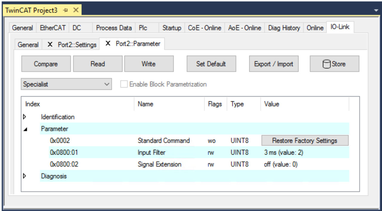
Fig. 18: Parameter of the device assigned to port2
