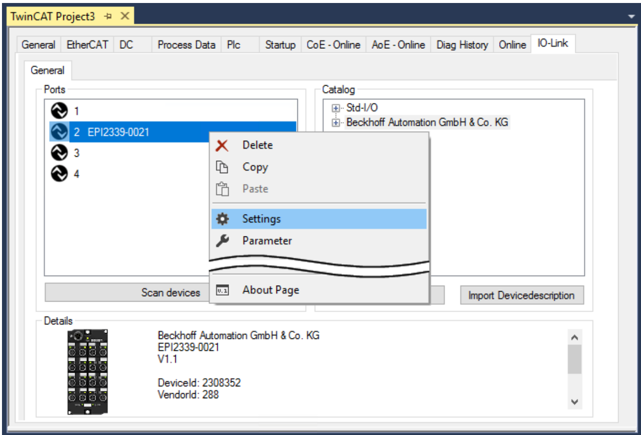
Fig. 16: Device at Port2, Display “Details”, open tabs “Settings” and “Parameter”
