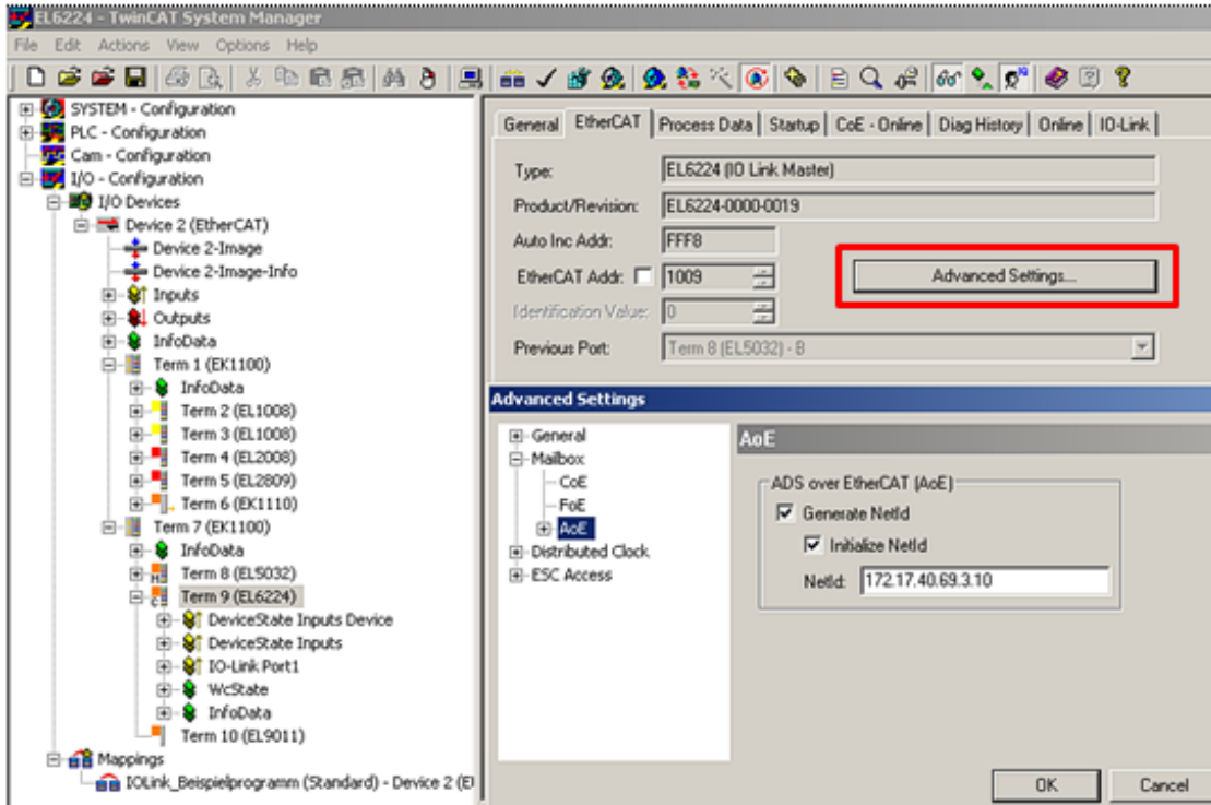
Fig. 38: AoE-NetID allocation
