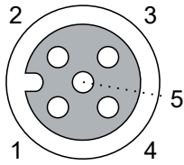
Fig. 13: M12 socket, 5-pin
