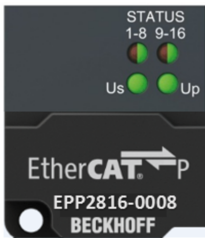
Abb. 6: EPP2816-0008 - Status-LEDs
