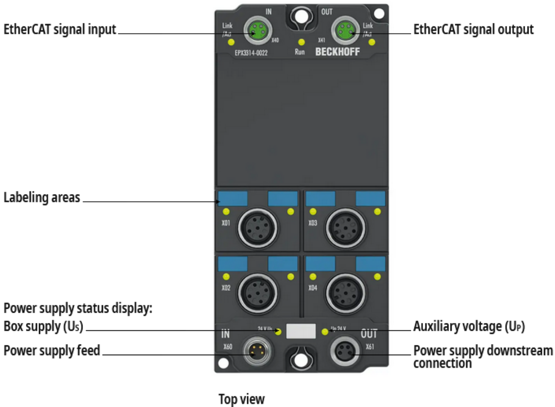
Fig. 2: EPX3314-0022 - EtherCAT Box, 4-channel analog input, thermocouple, 16-bit, M12, Ex i
