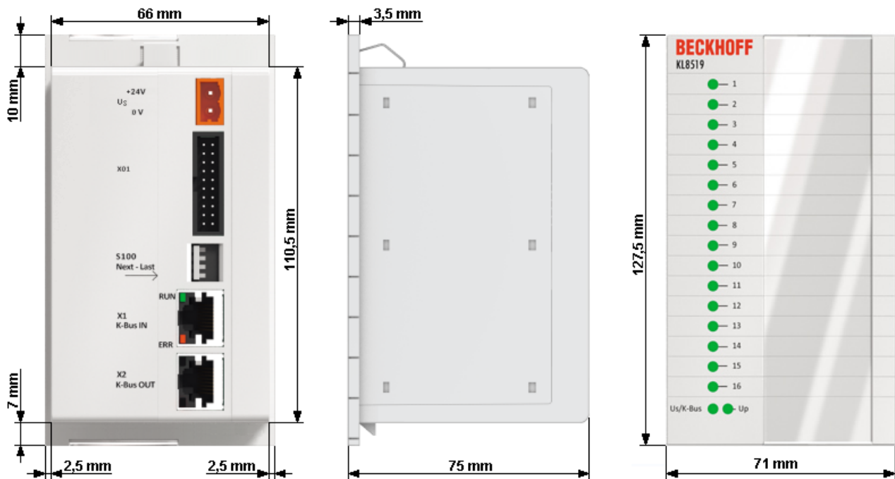
Fig. 11: Dimensions
