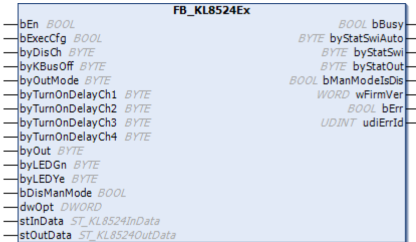
Fig. 26: Function block FB_KL8524Ex
