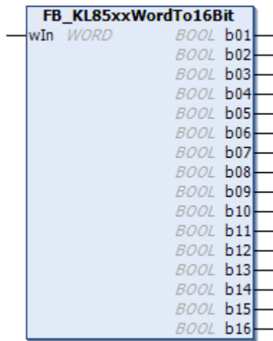
Fig. 34: Function block FB_KL85xxWordTo16Bit
