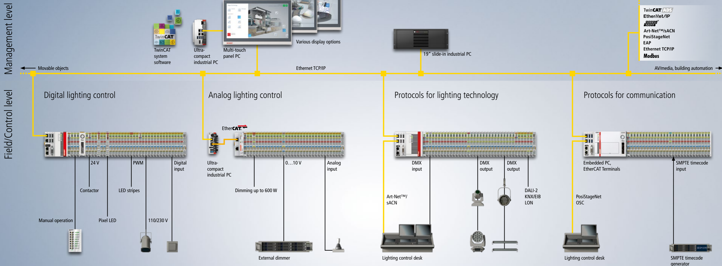
Technical functional drawing
