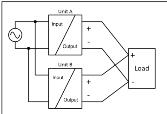
Fig. 22: Parallel connection
