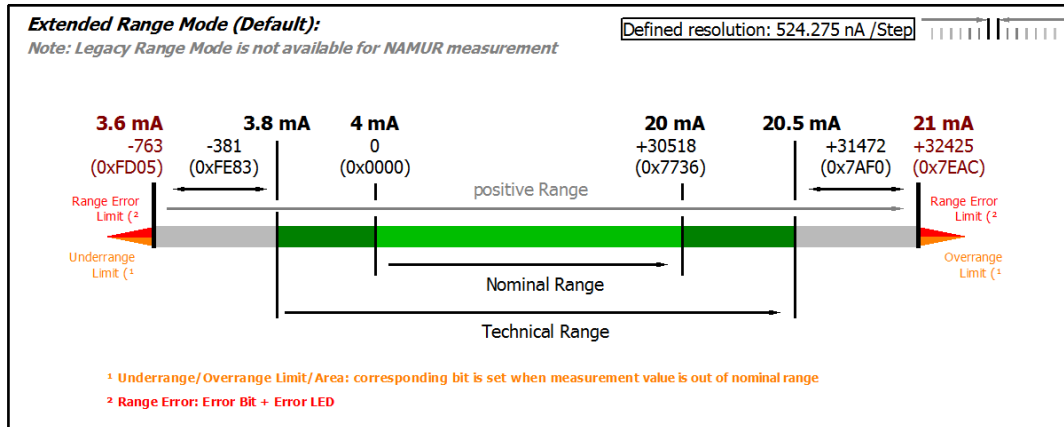
附图 153: ELX315x - 测量范围4...20 mA (NAMUR NE43)
