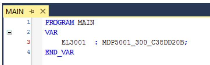
附图 72: Instance_of_struct
