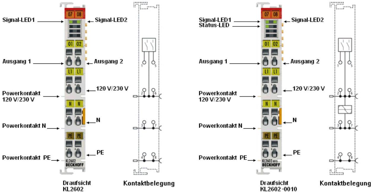
Abb. 1: KL2602-0000, KL2602-0010
