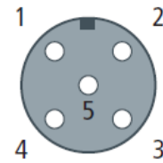
M12, socket, 5-pole
