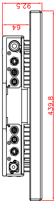
bottom view
