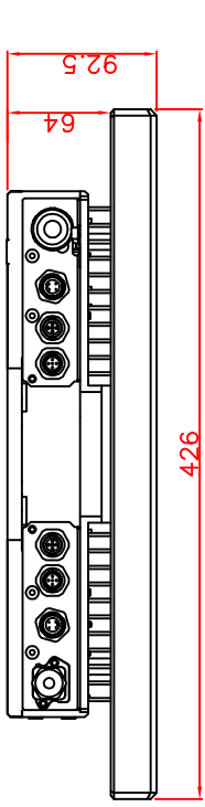
bottom view
