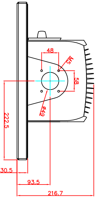
top view
