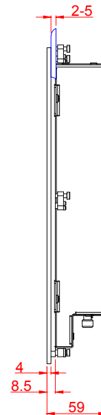
left view
