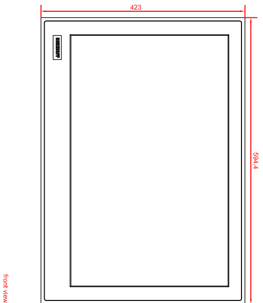
CP6204-0000-0030 main dimensions
