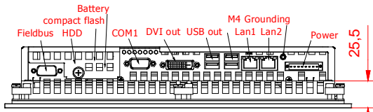
bottom view
