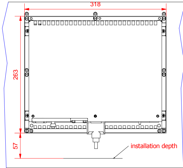
rear view with install measure
