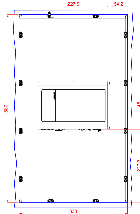
rear view
