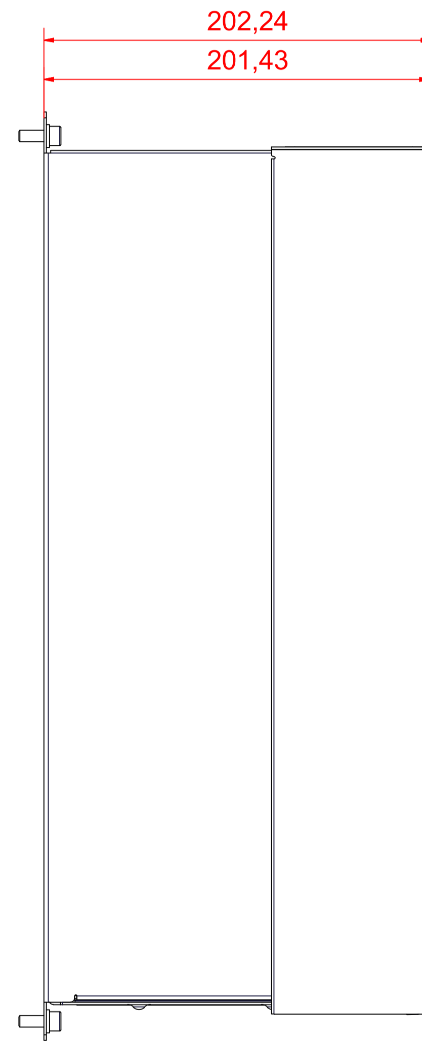
left view
