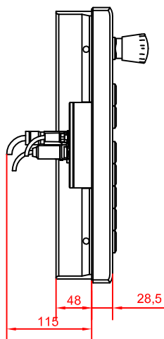
left view
