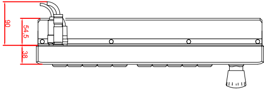
left view
