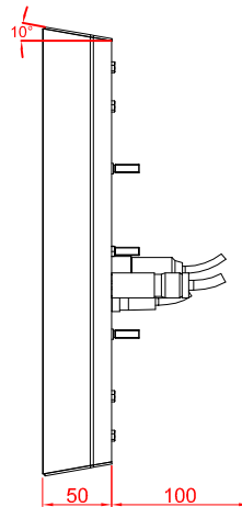
right view
