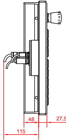
left view
