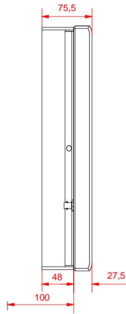
installation depth cp-link connectors left view
