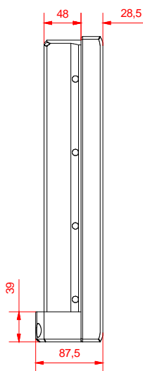
left view
