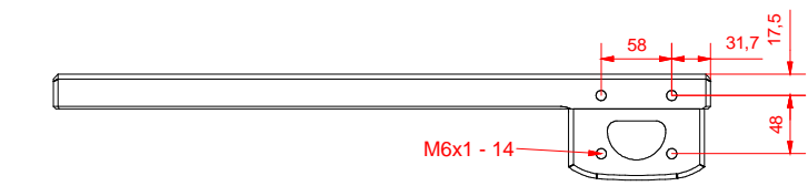
bottom view
