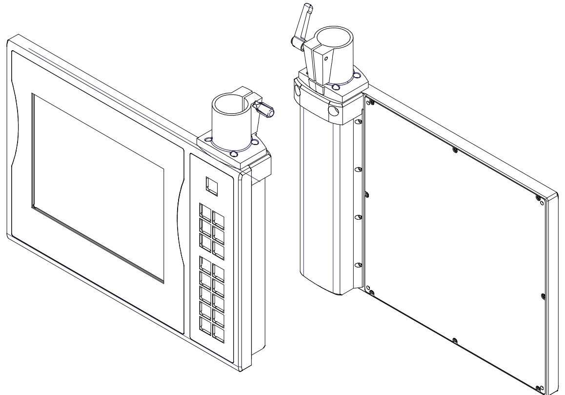
left view
