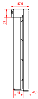
left view
