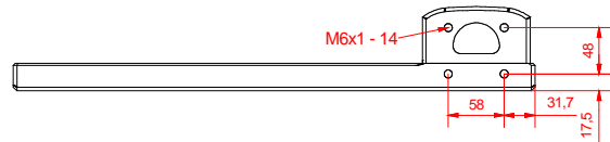
top view
