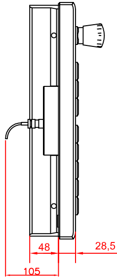
left view
