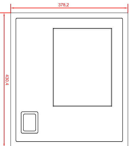
CF6931-0002 main dimensions
