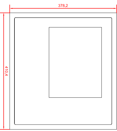
CP933 1-0000 main dimensions
