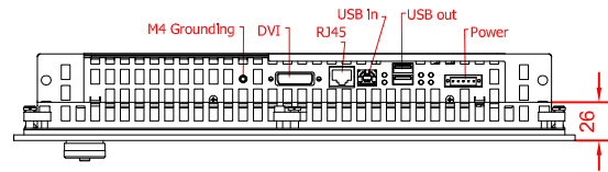
bottom view
